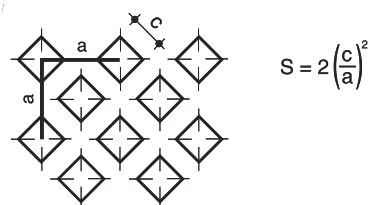
FORI QUADRI IN DIAGONALE E ALTERN. DIAGONAL SQUARE HOLES TROUS CARRÉS DIAGONAUX
