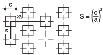
FORI QUADRI ALTERNATI STAGGERED SQUARE HOLES TROUS CARRÉS ALTERNÉS
